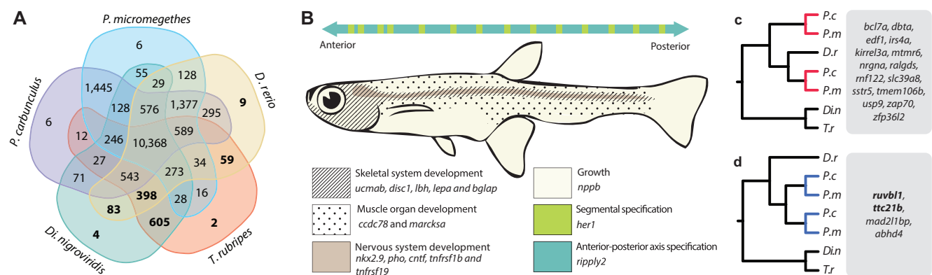
Fig. 2. —Gene loss and duplication of developmental process genes. (a) Five-species comparison of shared orthogroups for the identification of genes lost in Paedocypris . Bold numbers represent orthogroups without any Paedocypris orthologs. Orthogroups were identified using OrthoFinder (Emms and Kelly 2015) on the basis of full protein data sets for all included species. (b) Lost developmental pathway genes and schematic representation of phenotypically affected body segments in Paedocypris . (c) Gene duplicates retained in Paedocypris . (d) Genus-specific gene duplications. Genes in bold are associated with a truncated phenotype in Danio rerio .
